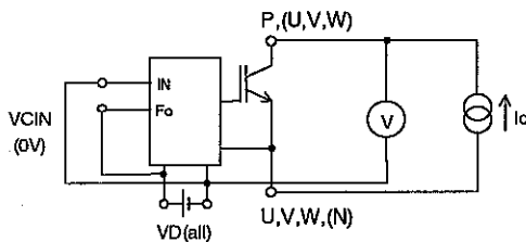
Fig.1 V CE(sat) Tset
